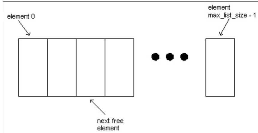
Figure 5-4 Implementing a List as an Array
